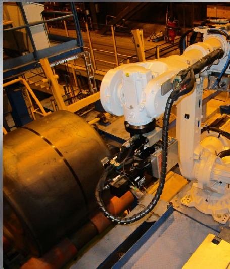
Destrapping Including High Strength Steel Straps
