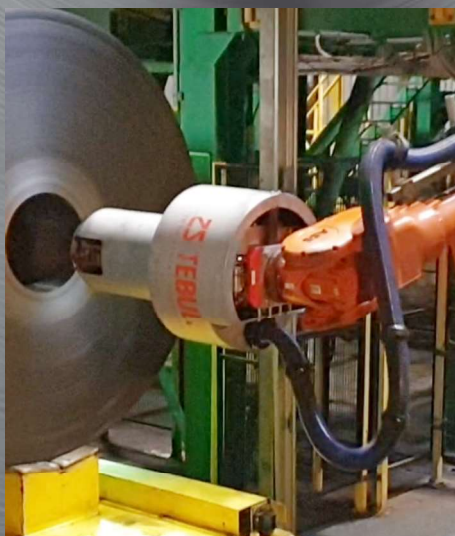
Coil Eye Welding
